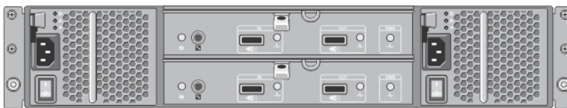
Figure 3. Dell PowerVault MD1200 Rear Chassis
